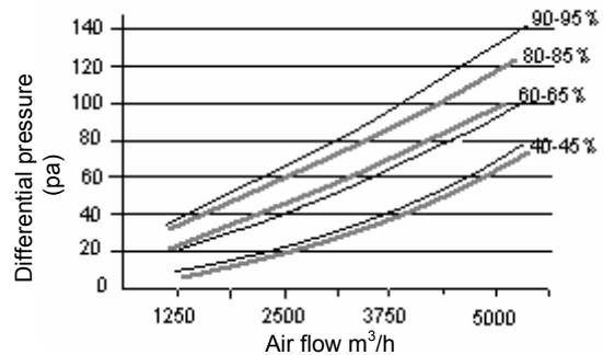
Air flow vs. differential pressure For size 592x592x292 mm
